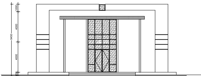
ELEVATION -E1 SCALE 100
