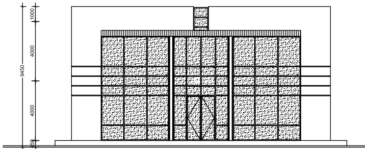
ELEVATION -E3 SCALE 100
