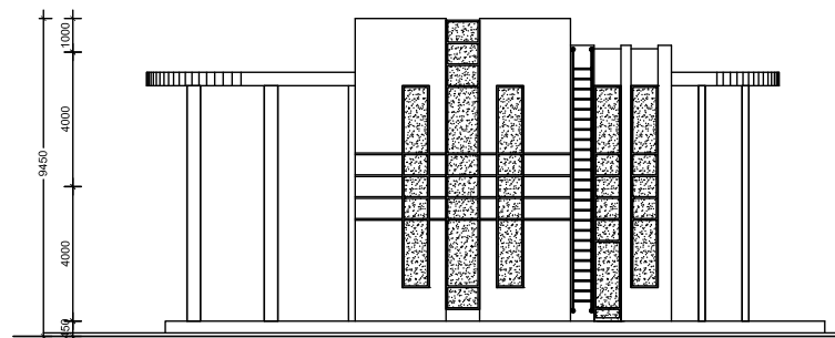
ELEVATION -E2 SCALE 100
