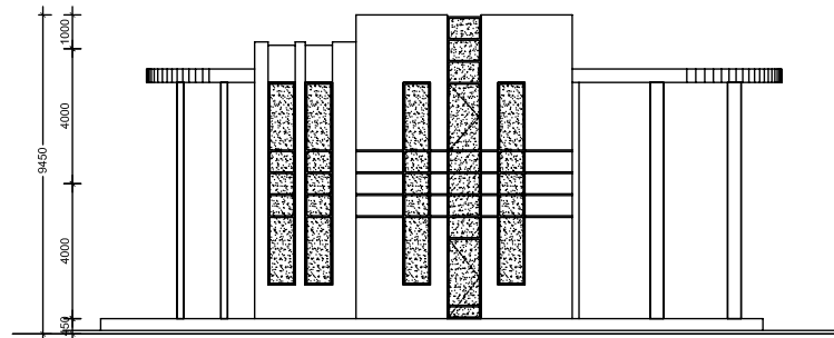
ELEVATION -E4 SCALE 100
